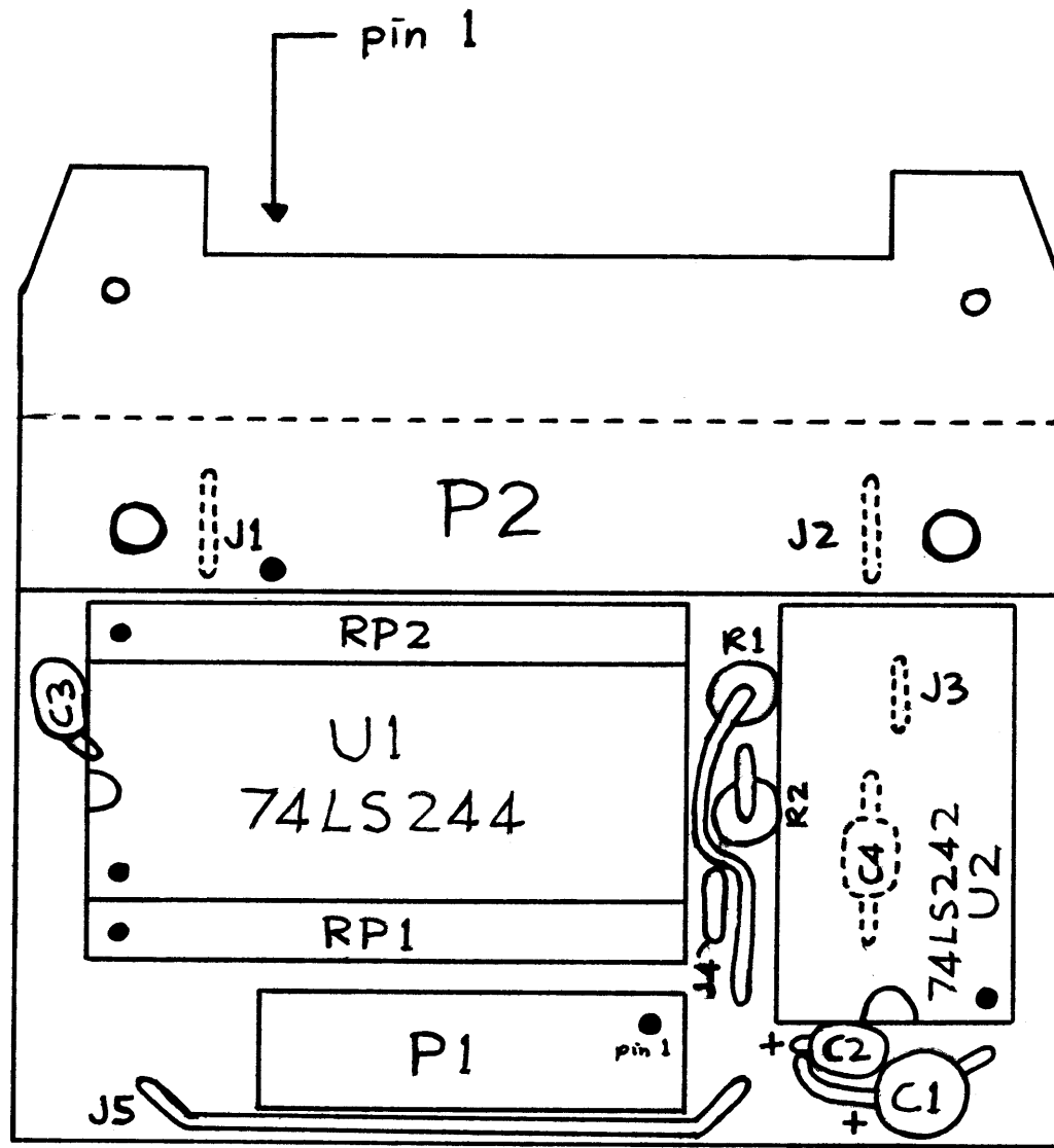
CNT-1 Component Layout
